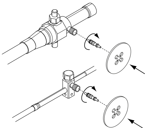
Figure 19. Replace pressure tap valve cores and plastic tabs
