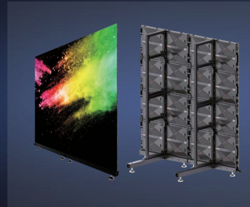
Stacking Installation
