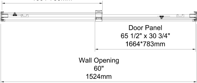
Door Panel 65 1/2" x 30 3/4" 1664*783mm
