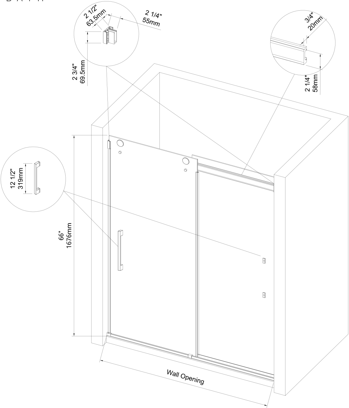
Door Panel 65 1/2" x 30 3/4" 1664*783mm
