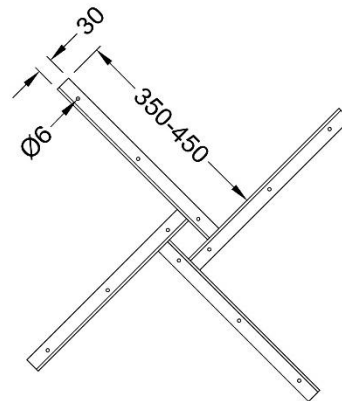
Cross (30mm x 30mm x 5mm Angle Bar) Suit Tops more than 900mm Dia
