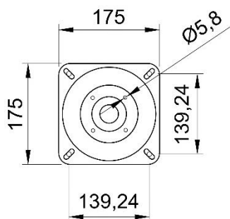
Swivel Top Mechanism
