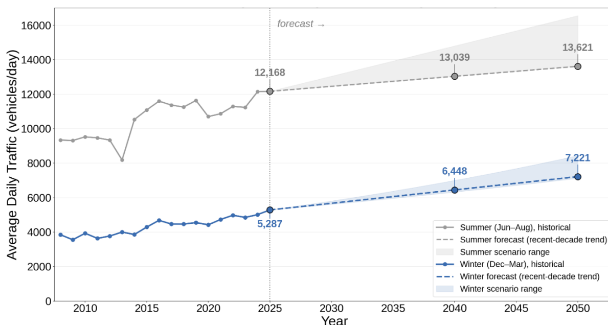
Figure 1: Winter average daily traffic (WADT) for the BC MOTT traffic count station at Craigellachie (site P-22-1EW) close to Three Valley Gap and possible future WADT scenarios until 2050. Winter forecast range spans three scenarios: full-history CAGR (2008–2025, 1.89%/yr, upper), recent-decade linear trend (2016–2025, central), and a 1.2%/yr 5-year CAGR (lower). Summer forecast range spans full-history linear trend, recent-decade linear trend, and recent-decade CAGR (2016–2025). Central dashed line = recent-decade linear trend. Winter (blue) = Dec–Mar monthly average; Summer (gray) = Jun–Aug monthly average.
