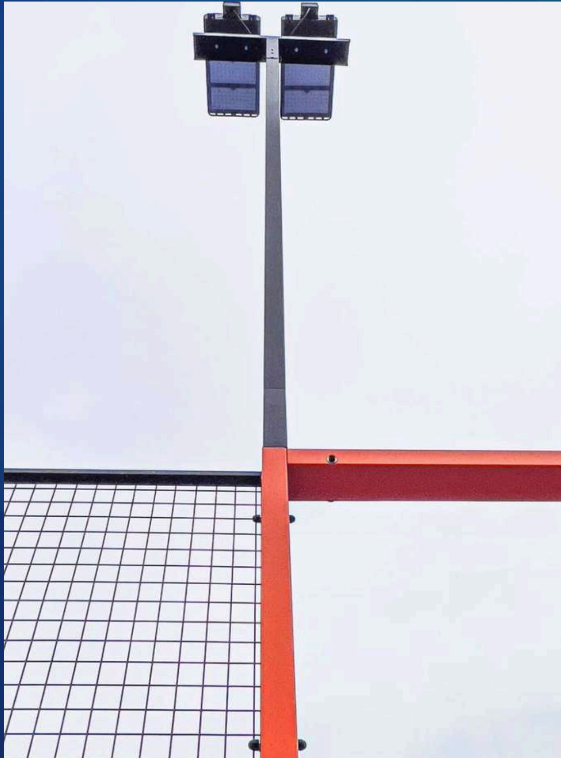
Robust welded LIGHT posts 100% integrated into the metallic structure. Avoid light vibration & failure
