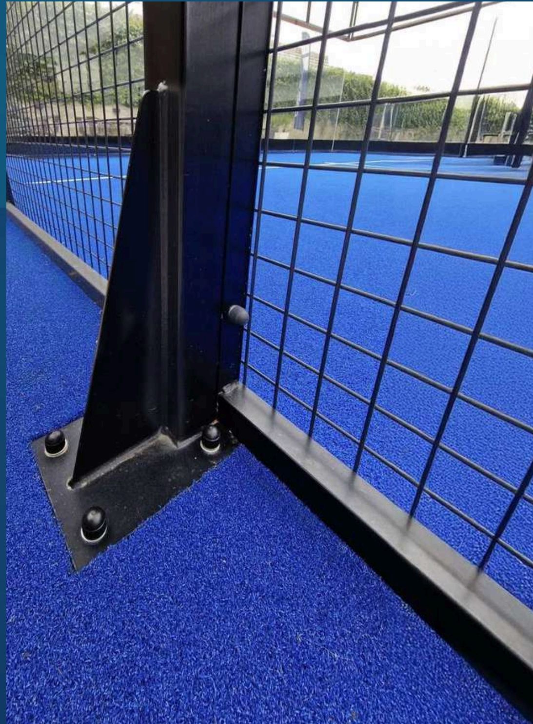
Robust welded MESH posts with big tube + large anchor plate + high rib. Avoid mesh vibration & noise
