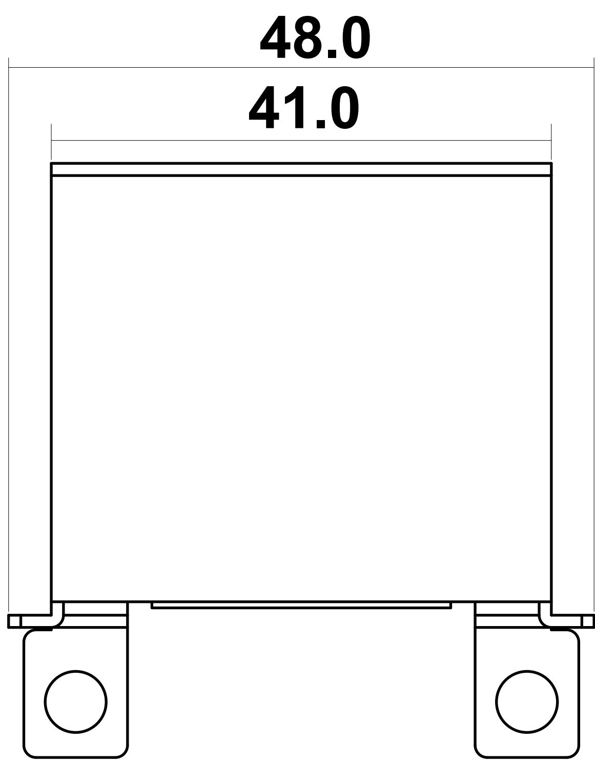
5 TOP VIEW
