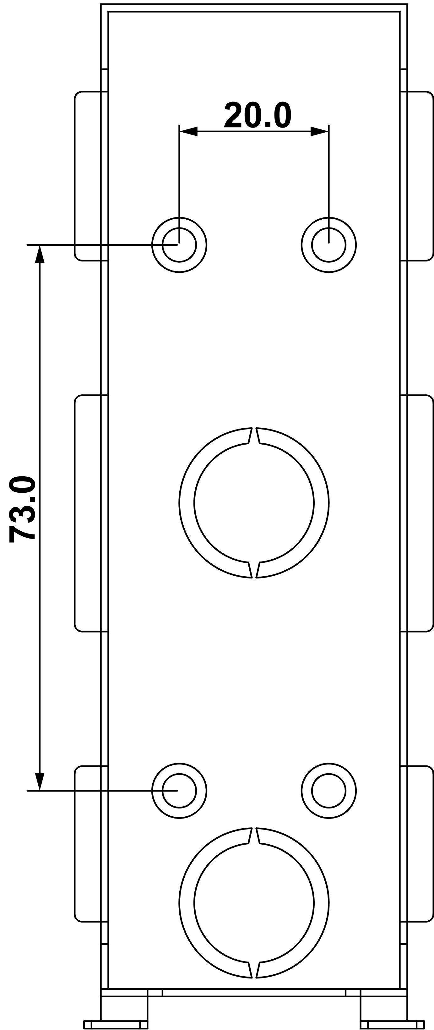
6 BOTTOM VIEW
