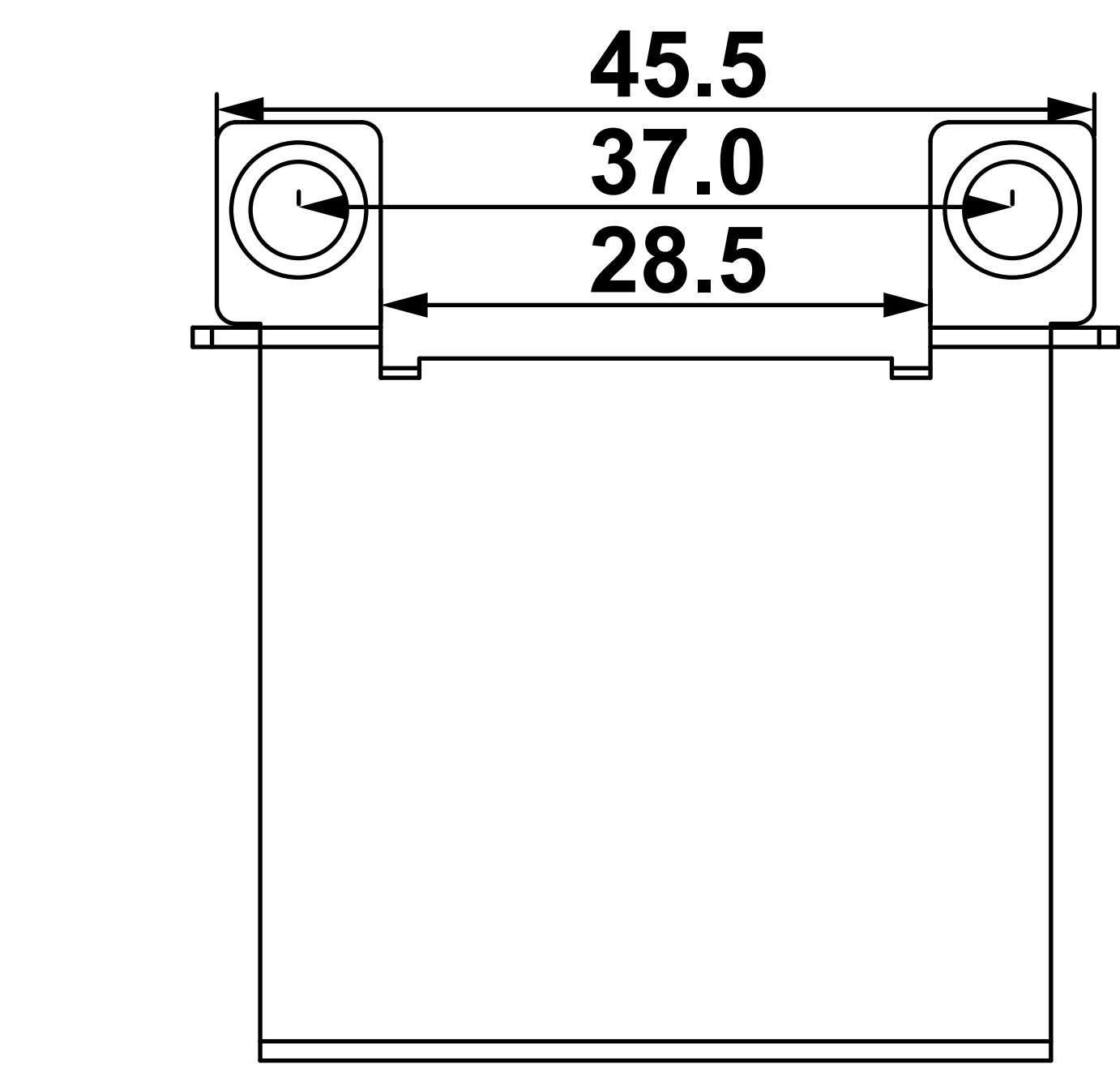
6 BOTTOM VIEW
