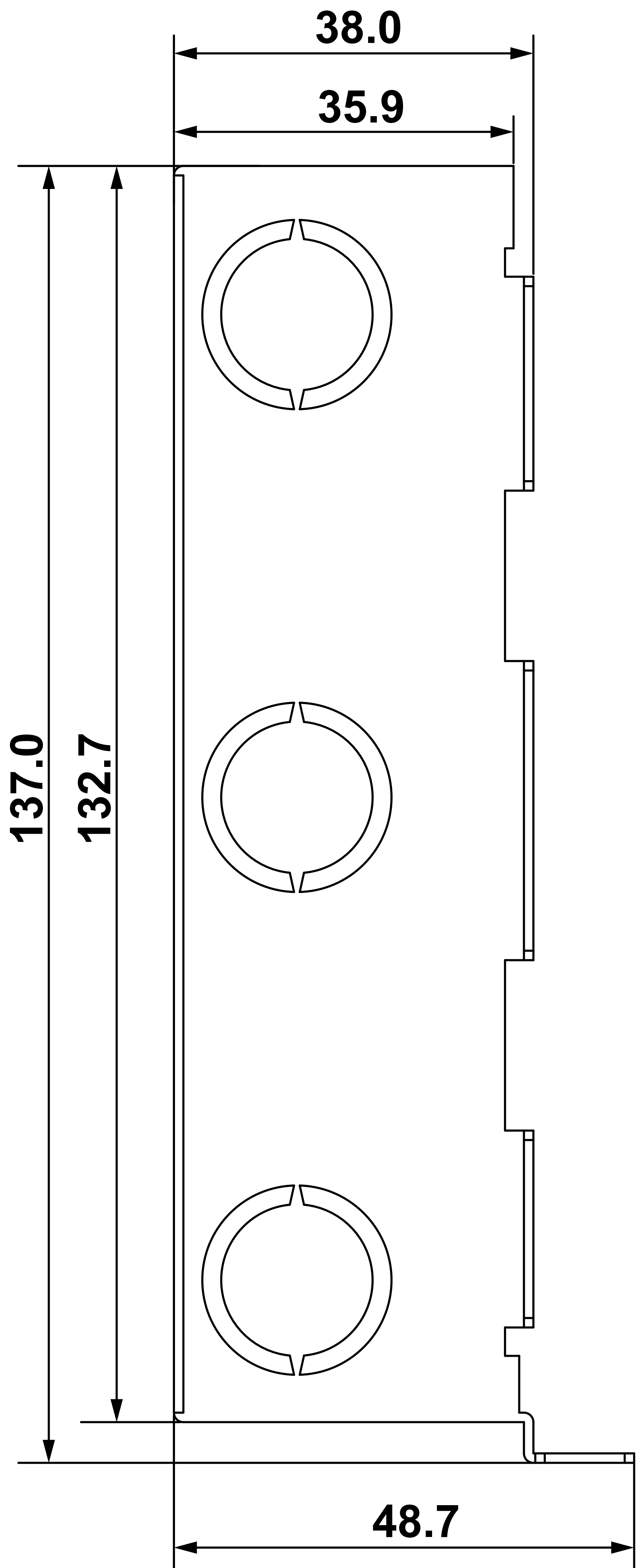
3 LEFT VIEW
