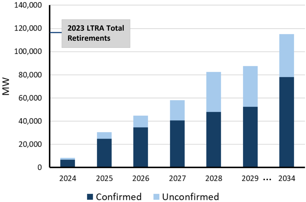
Figure 14: Projected Generation Retirement Capacity through 2034
