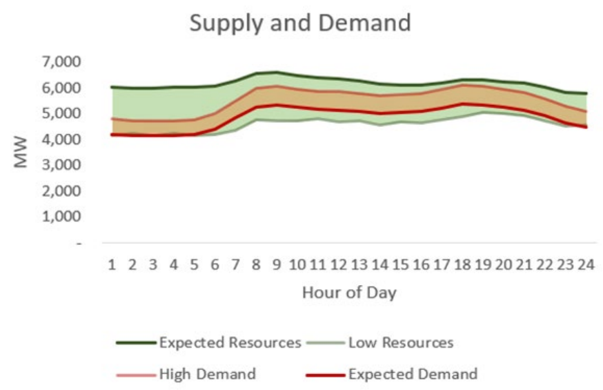
Hourly Probabilistic Assessment Results | Representative Summer Risk Day 2026
