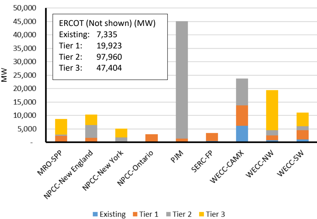
Figure 12: Battery Resource Capacity Existing and Planned through 2034
