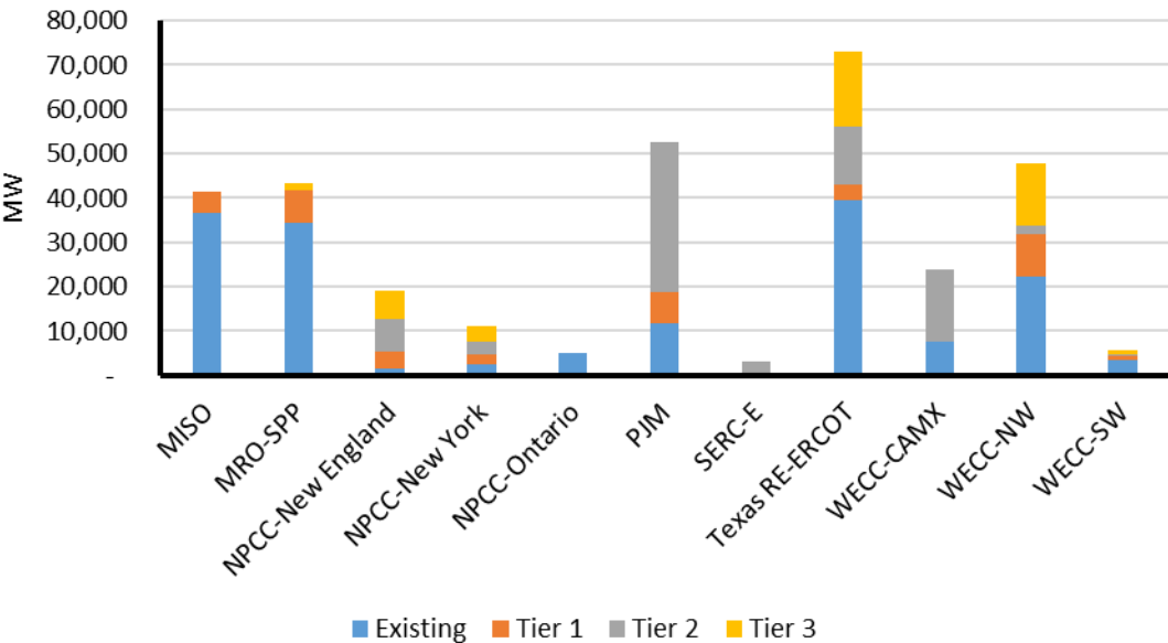
Figure 10: Wind Nameplate Capacity Existing and Planned through 2034
