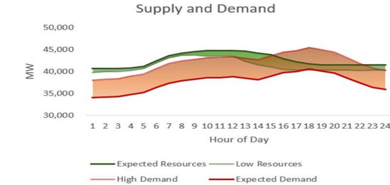
Hourly Probabilistic Assessment Results | Representative Winter Risk Day 2026
