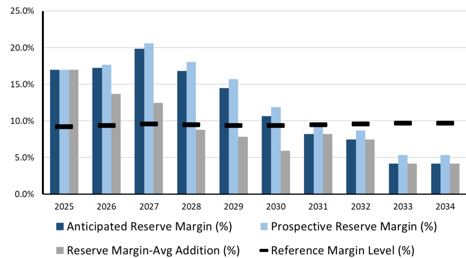
Figure 3: MISO Planning Reserve Margin–Summer
