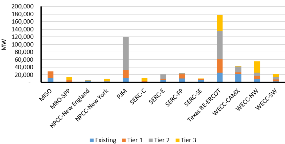
Figure 9: Solar Nameplate Capacity Existing and Planned through 2034
