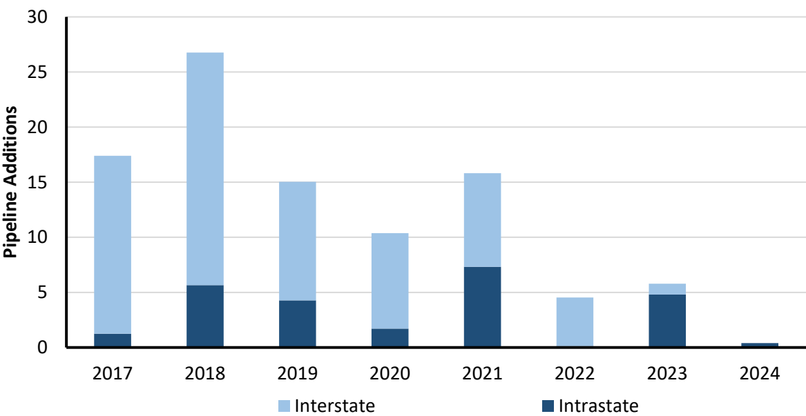
Figure 16: Annual U.S. Natural Gas Pipeline Capacity Additions by Type (2017–2024) Bcf/d (Source: U.S. Energy Information Administration)
