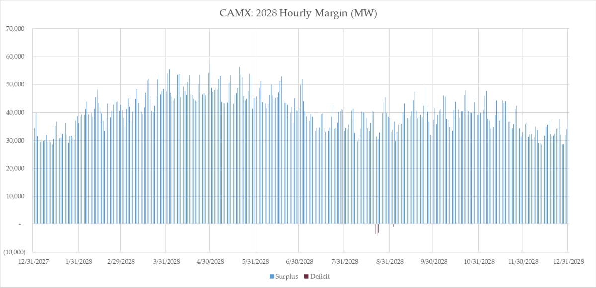
Icicle Plot with Hourly Surplus and Deficits for CA/MX in 2028
