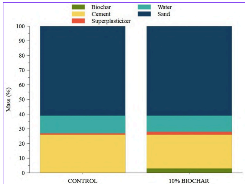
Caption: An example showing ratios of how a mortar mix may be adjusted in order to maintain workability. This example shows a 10% addition of biochar, maintaining a 0,45 water-to-cement mass ratio with approximately 1% of superplasticizer. From Relevant biochar characteristics influencing compressive strength of biochar-cement mortars by Hylton J, et al. and used under A CC BY 4.0 license.
