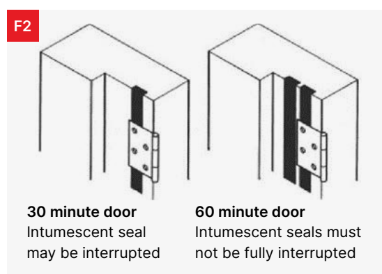
Figure 1: Typical seal arrangement of pressure generating intumescent seal concealed behind door lipping
