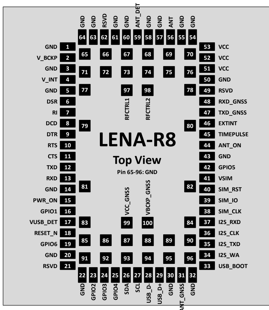
Figure 3: LENA-R8 series pin assignment (top view)
