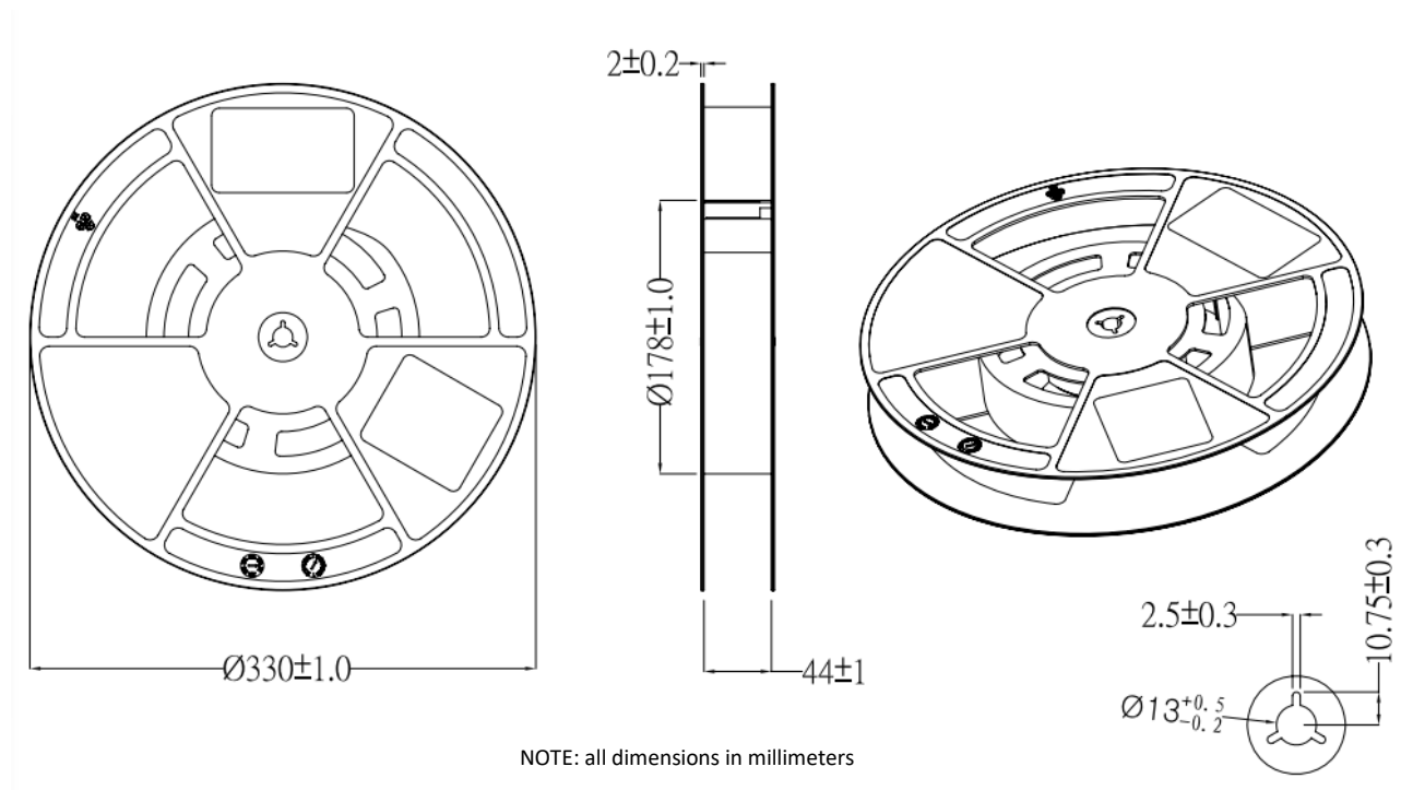
Figure 6: LENA-R8 series modules reel
