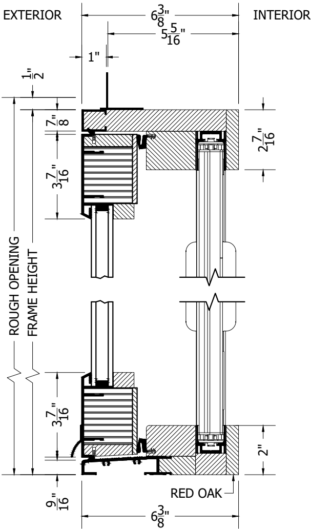
SECTION VIEW
