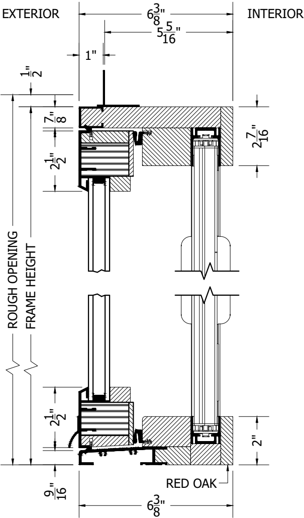
SECTION VIEW
