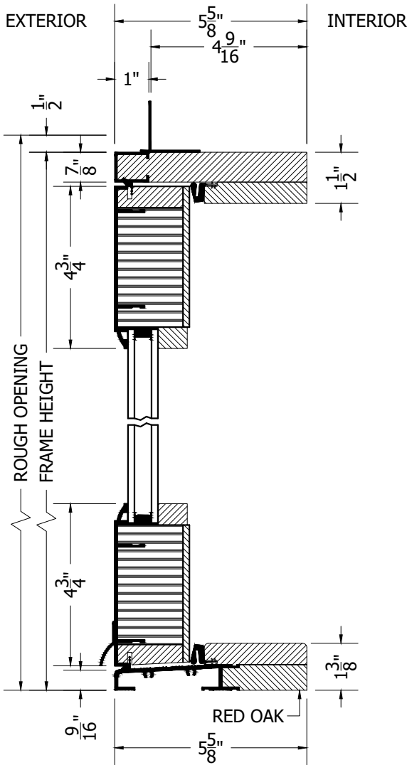
SECTION VIEW
