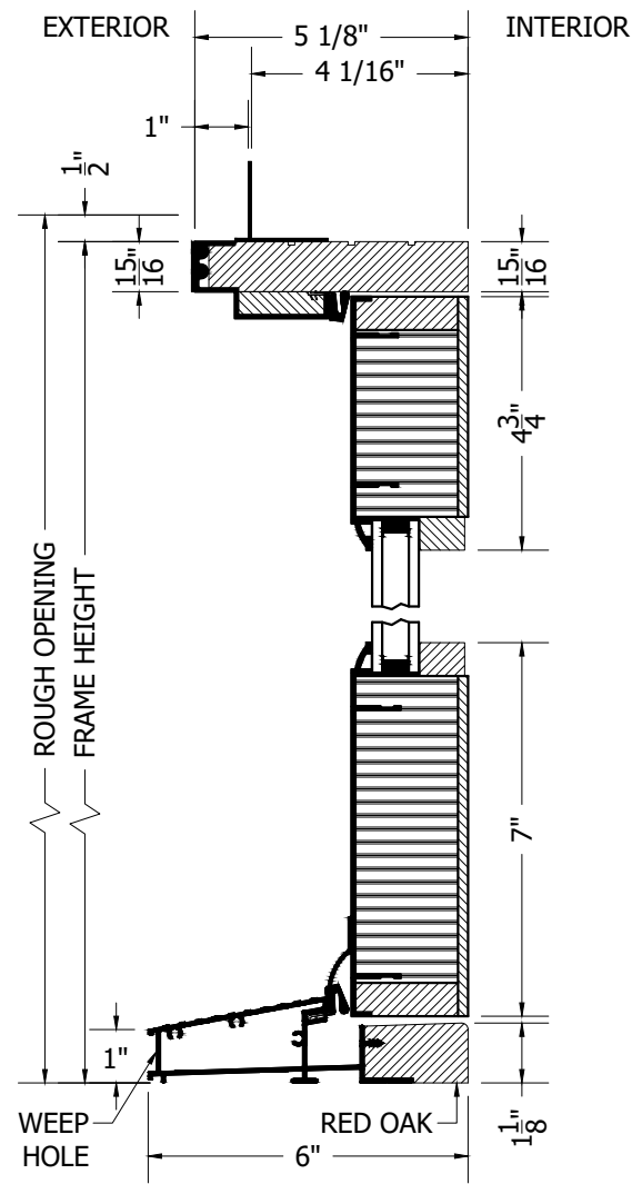
SECTION VIEW
