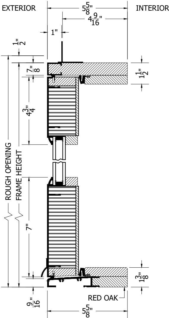
SECTION VIEW
