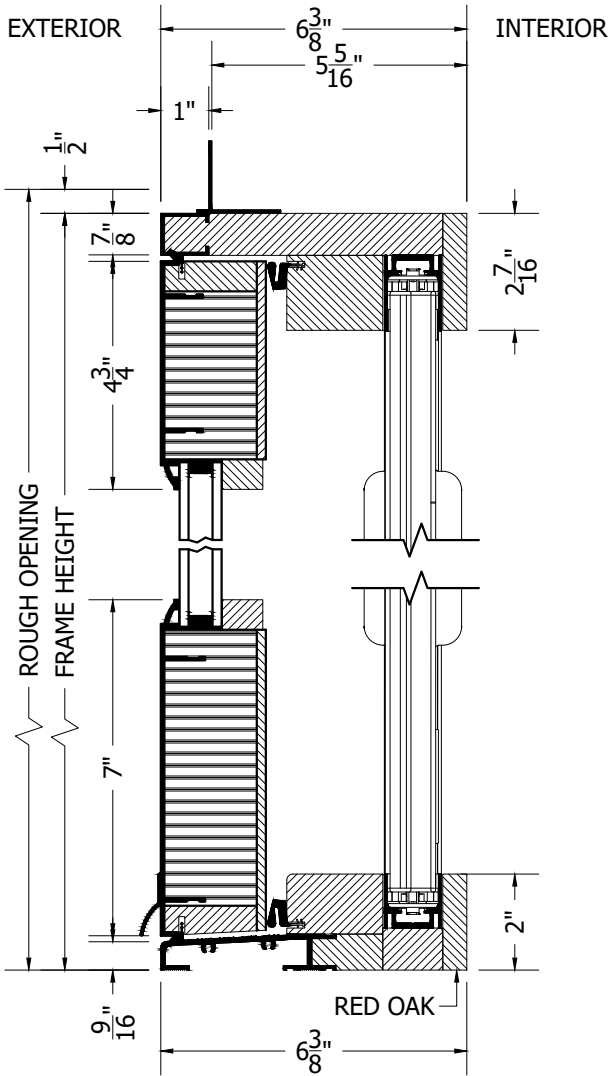
SECTION VIEW
