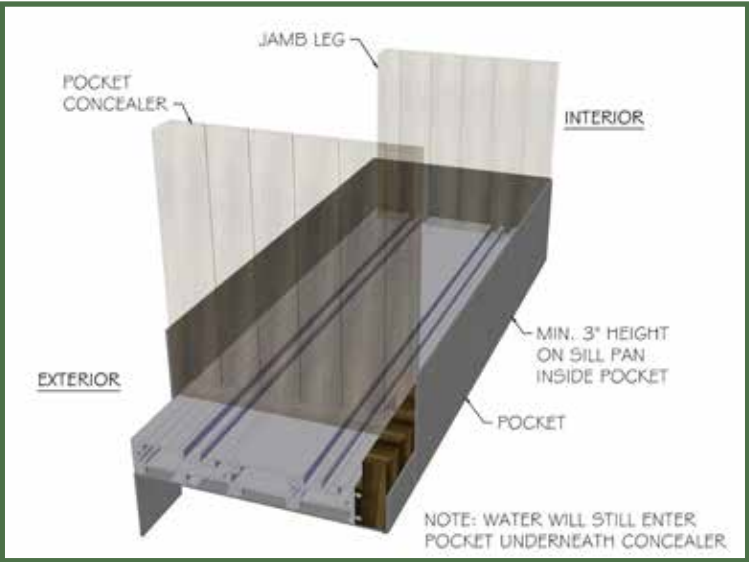
3-Sided Sill Pan for Pocket Sliders
