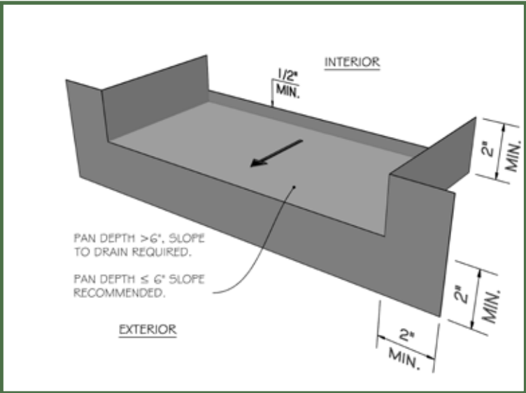
Standard Sill Pan Guidelines
