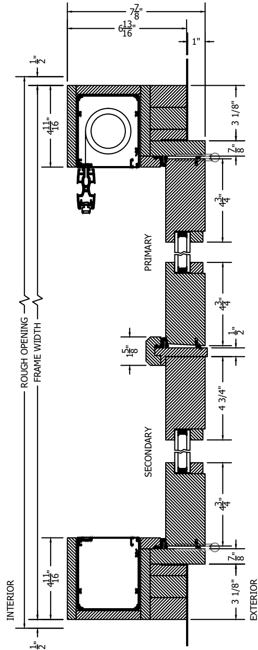
PLAN VIEW
