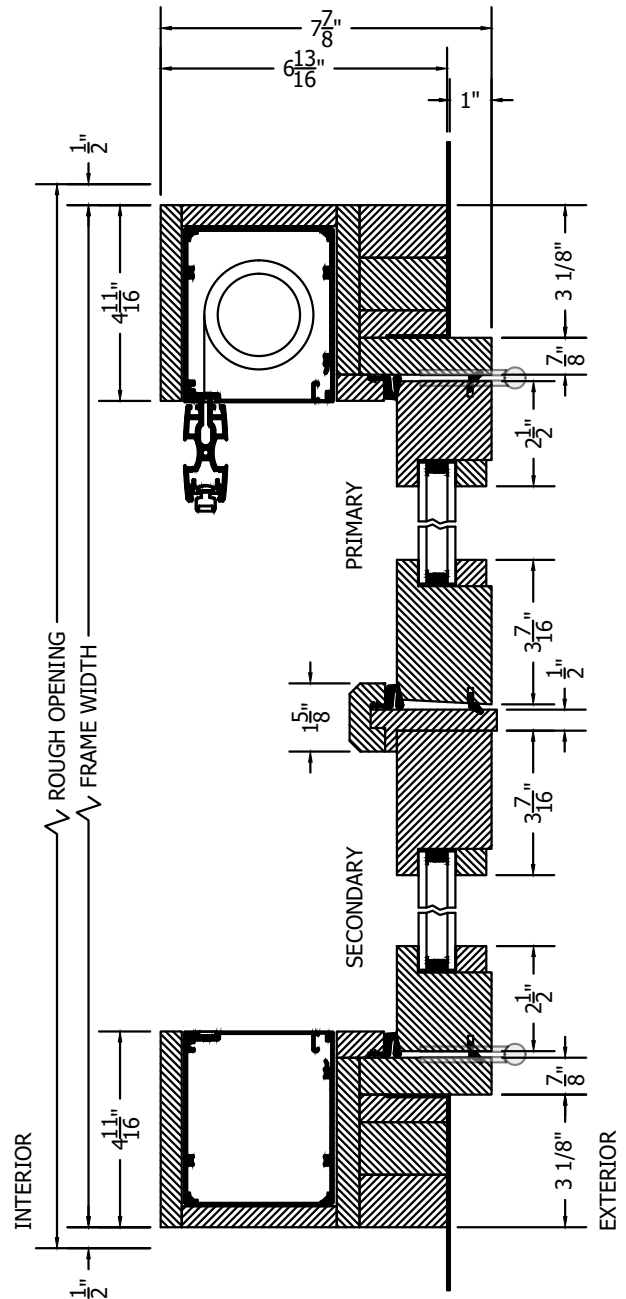
PLAN VIEW
