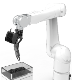
Bin-Picking Module
