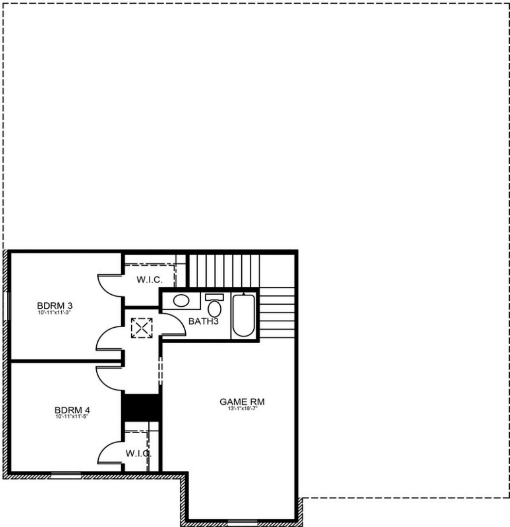
UPPER FLOOR - ELEVATION D
