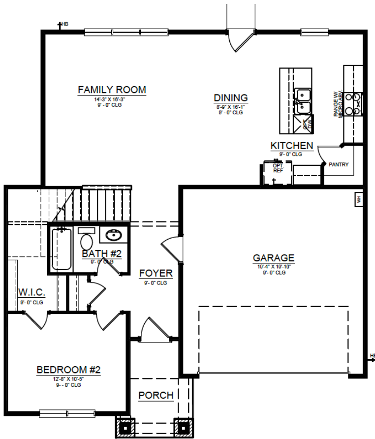
Craftsman Main Floor
