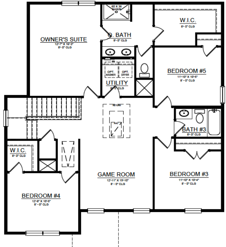
Craftsman Upper Floor
