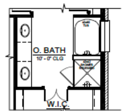
OWNERS BATH W/ SEPARATE TUB/SHOWER
