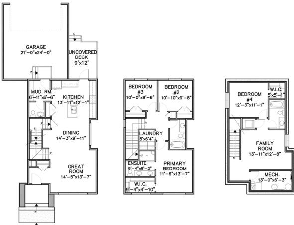
MAIN LEVEL FLOOR PLAN 763 sq. ft.
