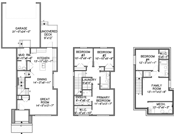
MAIN LEVEL FLOOR PLAN 763 sq. ft.
