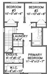
UPPER LEVEL FLOOR PLAN 719 sq. ft.
