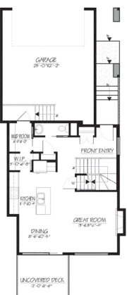
MAIN LEVEL 704 FT 2
