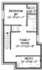
LOWER LEVEL 520 sq. ft.
