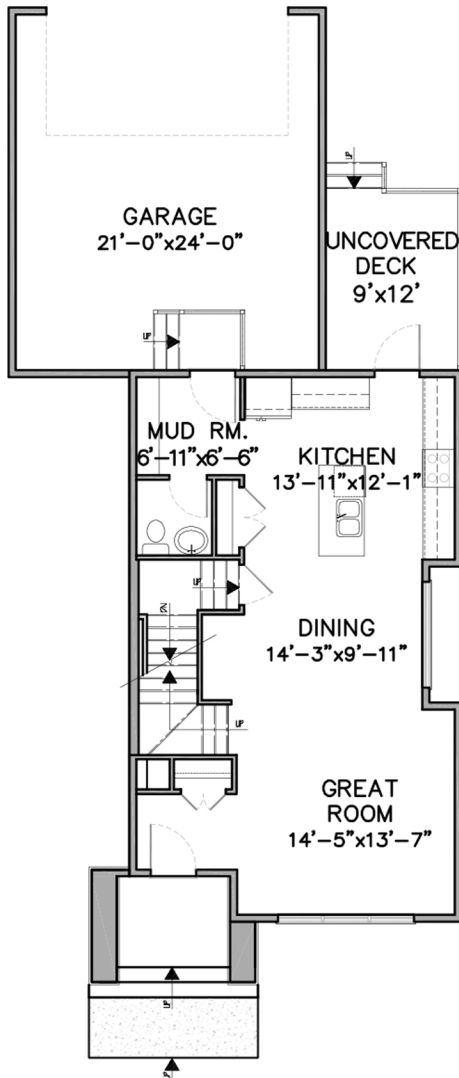
MAIN LEVEL FLOOR PLAN 763 sq. ft.
