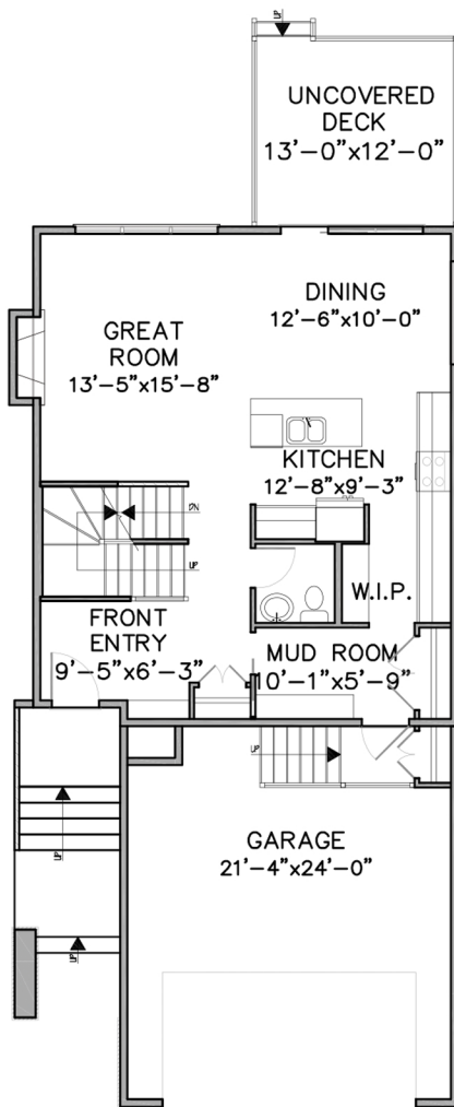
MAIN LEVEL FLOOR PLAN 838 sq.ft.
