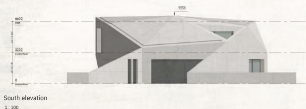
SOUTH ELEVATION
