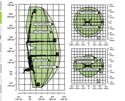
Range of Motion ZX23AE
