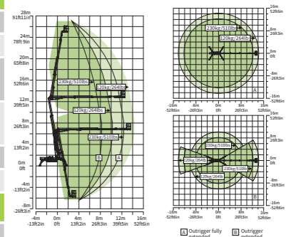
Range of Motion ZX27AE
