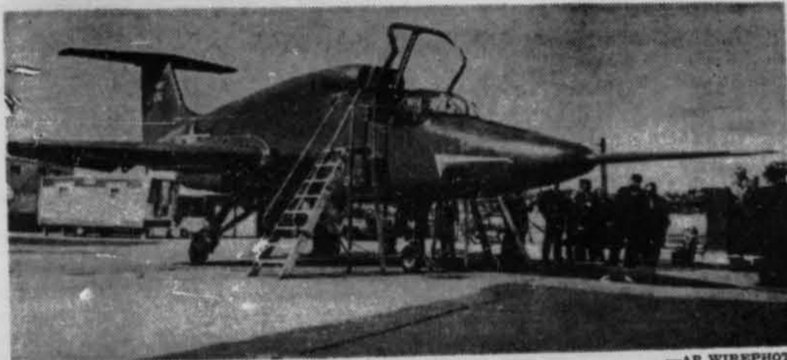
THIS IS a lift-fan jet, V-STOL, unveiled at Ryan Aeronautical Co., San Diego, Calif. It can take off vertically. The aircraft, built for the U.S. Army, can operate out of a field the size of a tennis court. It is still in experimental stage.
