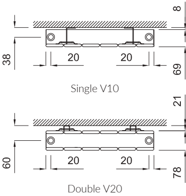
Slieve Vertical Plan
