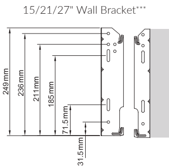
Bracket Plan View
