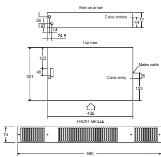
KICKSPACE® 80S
