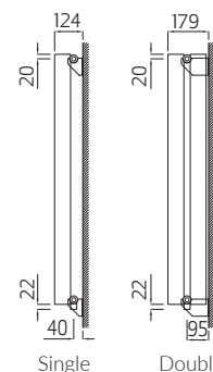
Adagio 70 Vertical Section
