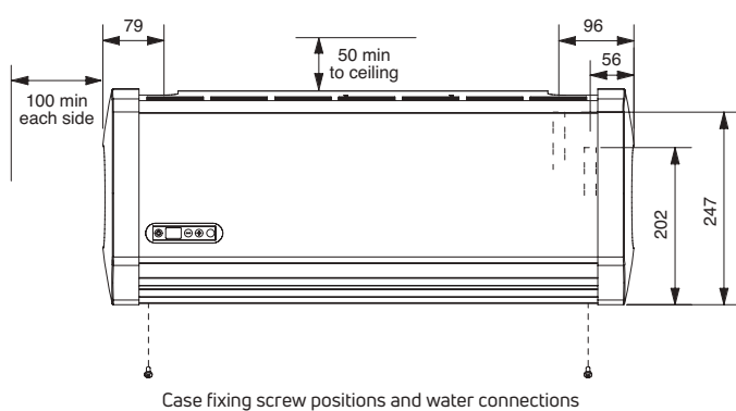
Case fixing screw positions and water connections
