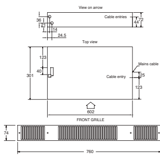
KICKSPACE® 80D
