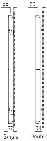
Slieve Vertical Section
