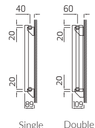
Adagio 35 Horizontal - Single and Double Section
