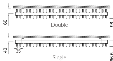
Adagio 35 Horizontal - Single and Double Plan
