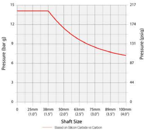
PV Chart
