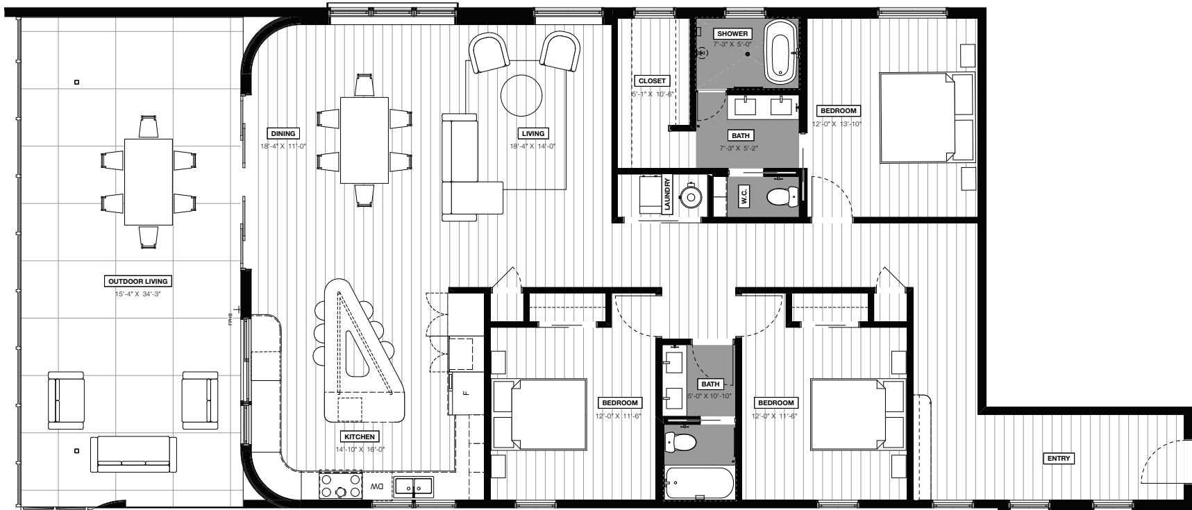
UNIT PLAN [3C] - 1880 SF
