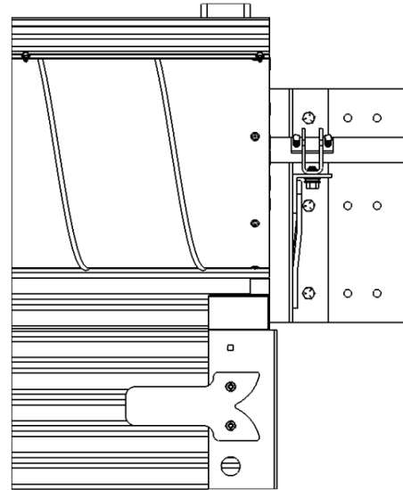
figure 21: Headstops
