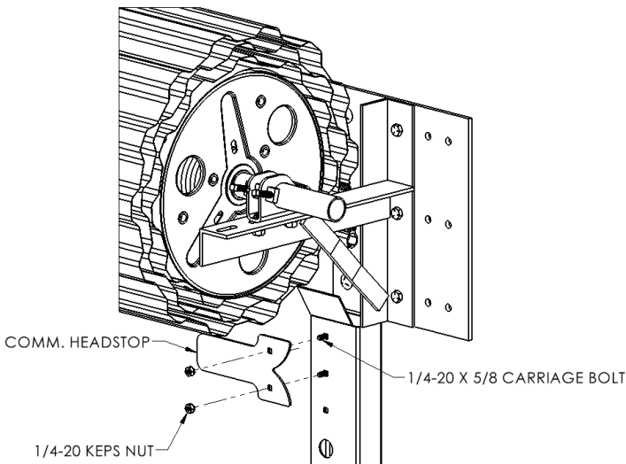
figure 20: Headstops
