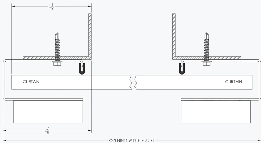
figure 17: Steel Jambs
