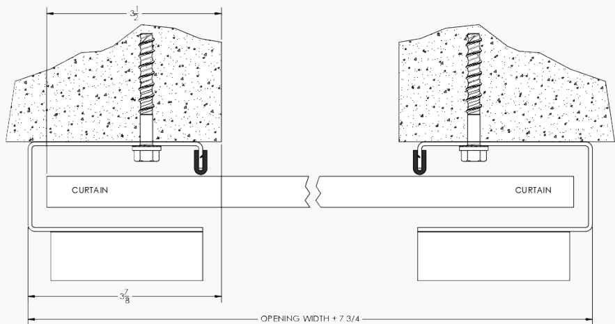
figure 18: Concrete / Masonry Jambs
