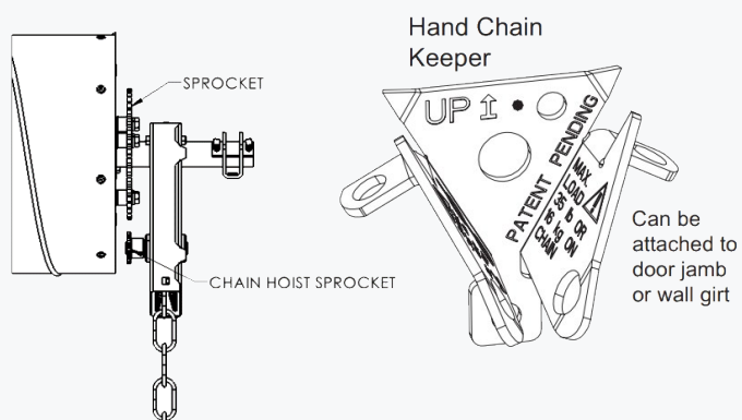
figure 14: Securing Stamped Axle Support w/ Chain Hoist (Curtain removed from illustration)
