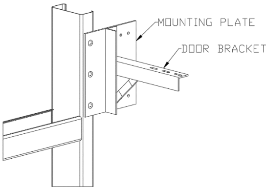
figure 7: Door Bracket to Mounting Plate
