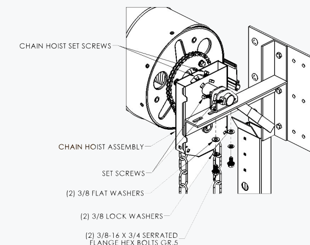
figure 14: Securing Stamped Axle Support w/ Chain Hoist (Curtain removed from illustration)
