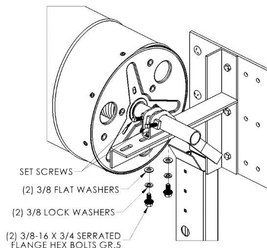
figure 13: Securing Stamped Axle Support (Curtain removed from illustration)
