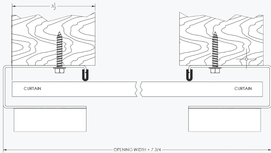
figure 19: Wood Jamb
