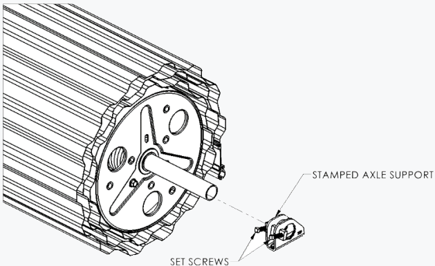
figure 8: Stamped Axle Support Installation
