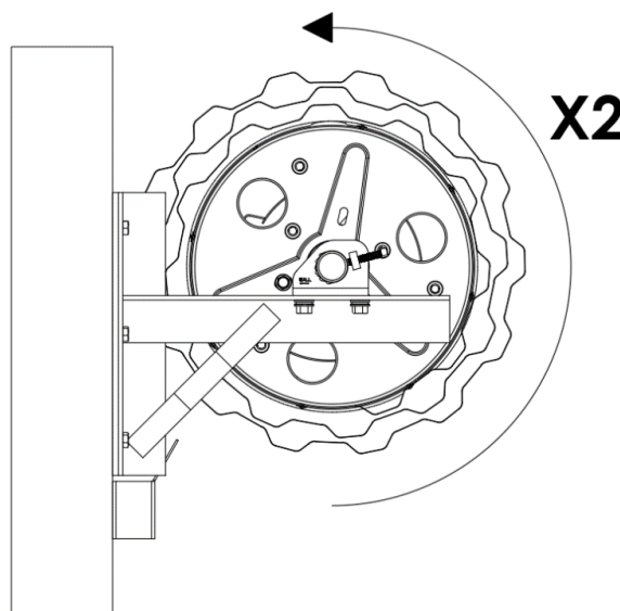
figure 16: Setting Initial Spring Tension
