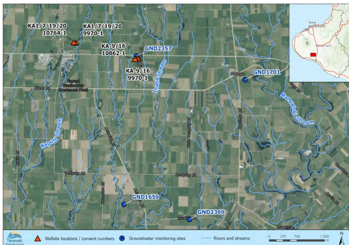
Figure 6.5 Location of monitoring sites at Kapuni (Skinner et al. 2013).
