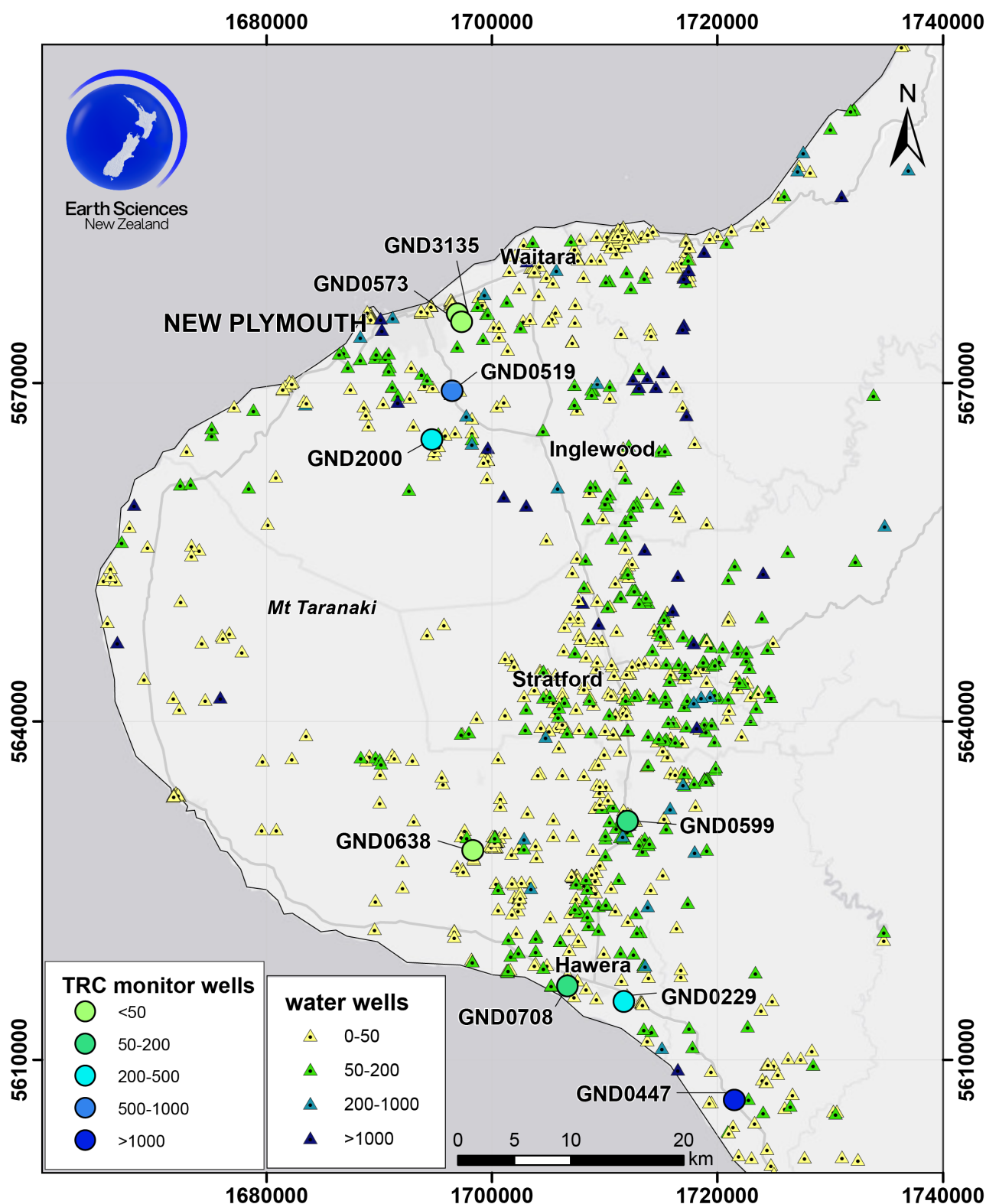
Figure 2.4 Locations of known Taranaki Regional Council water wells in Taranaki. Circles show the locations of wells, for a given depth, with monitored temperatures.
