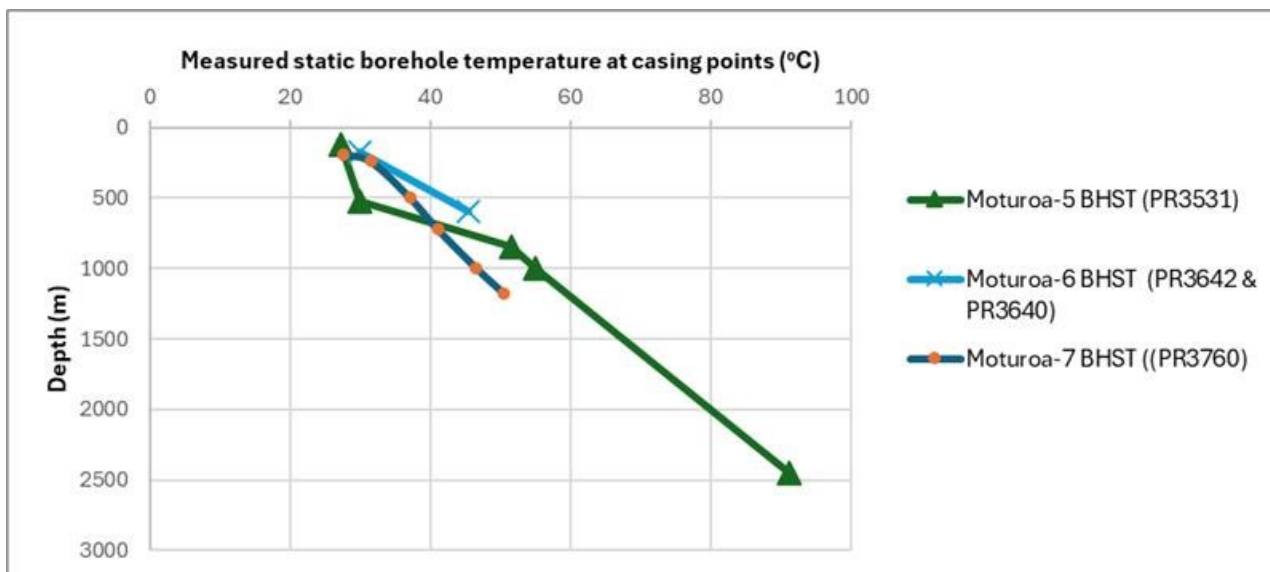
Figure 6.2 Plot of static temperatures measured at casing points in the borehole, provided by a cementing contractor (Haliburton).
