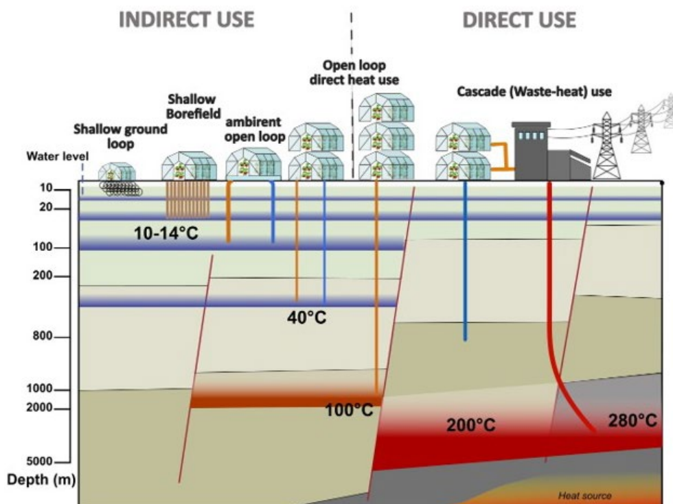
Figure 1.2 Schematic of subsurface conditions from which geoheat can be extracted.
