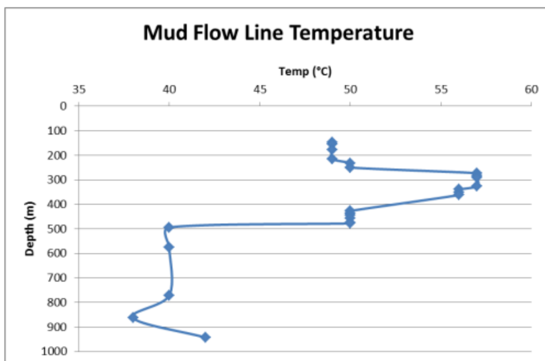
Figure 2.6 Temperature of mud in flow lines for Mauku-1 through the shallow sedimentary section (from Skinner et al. 2013).
