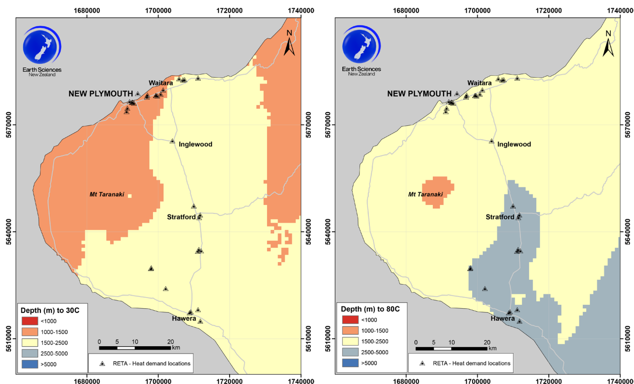
Figure 2.8 Modelled depth to a defined temperature for the Taranaki region. Left: Modelled subsurface depths at which 30°C is reached, with the locations of Taranaki heat users shown (EECA 2025); Right: Modelled subsurface depths at which 80°C is reached, with the locations of the Taranaki heat users shown (EECA 2025).
