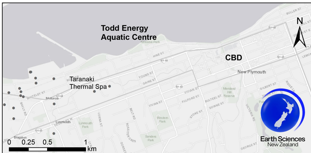
Figure 6.1 Location of Todd Energy Aquatic Centre and the Taranaki Thermal Spa. Petroleum wells associated with Moturoa Field near Taranaki Port are shown by grey dots.
