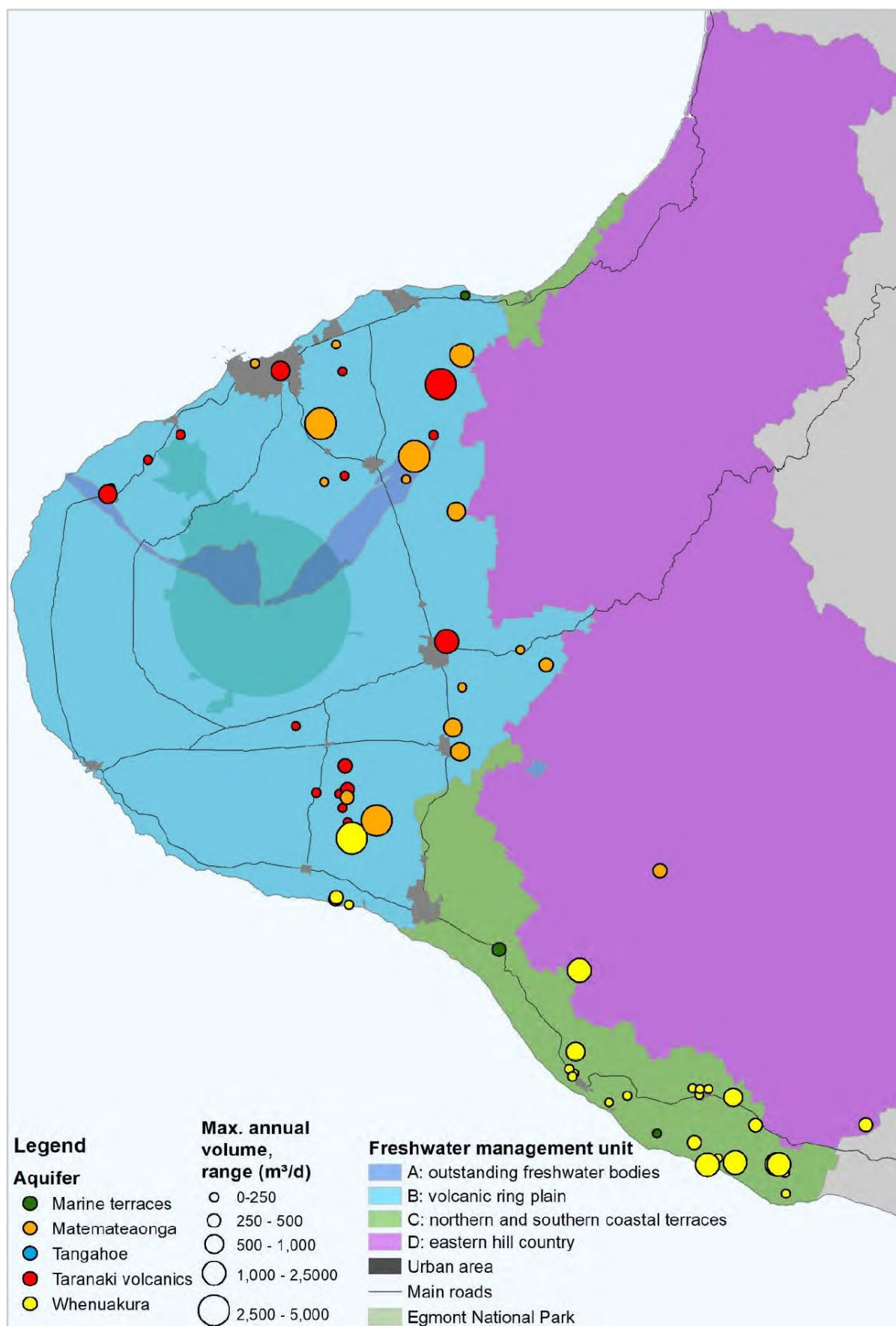
Figure 2.3 Hydrological units in Taranaki (Taranaki Regional Council 2018). Circles show the locations of consented groundwater extraction (as of June 2017), colours indicate the unit from which these are extracting and size indicates the volume.
