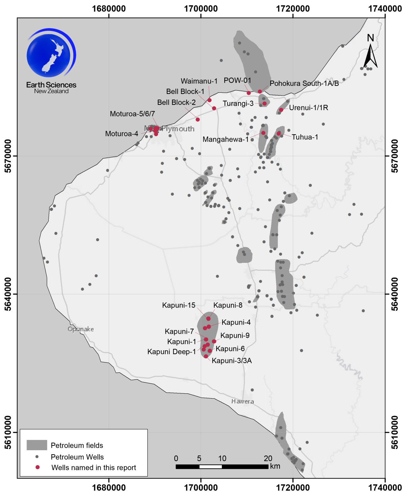
Figure 2.5 Locations of all known petroleum boreholes in the Taranaki region. Boreholes marked in red are used in the case-study areas in Section 6.
