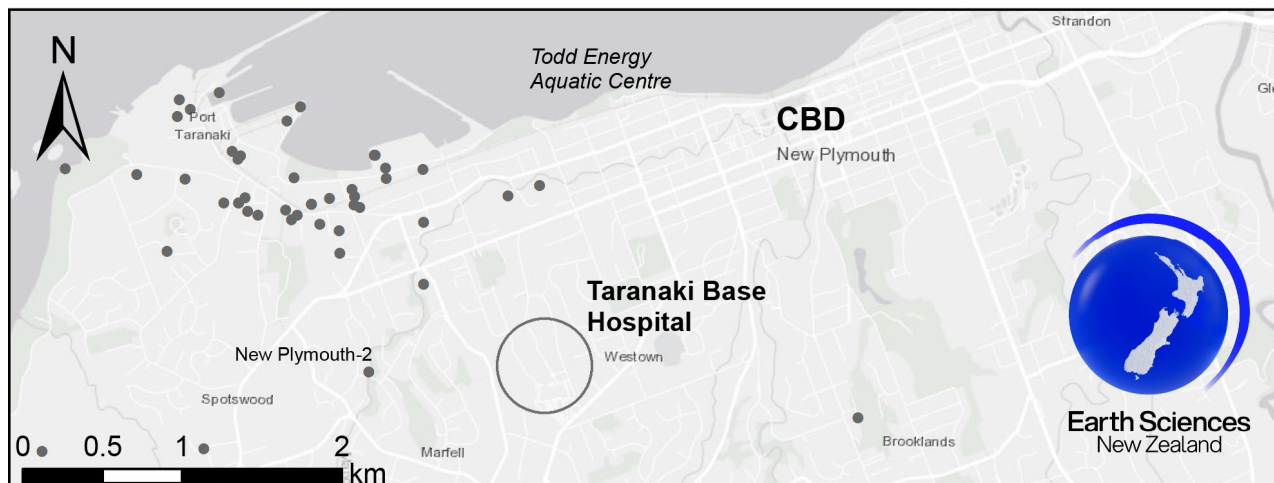
Figure 6.3 Location of Taranaki Base Hospital and nearby petroleum wells of Moturoa Field.
