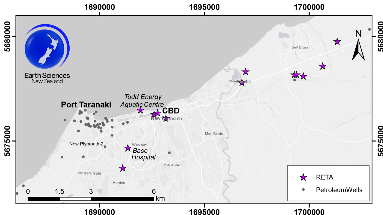
Figure 6.6 Location of petroleum wells (grey dots) and heat users (purple stars) in the New Plymouth area.
