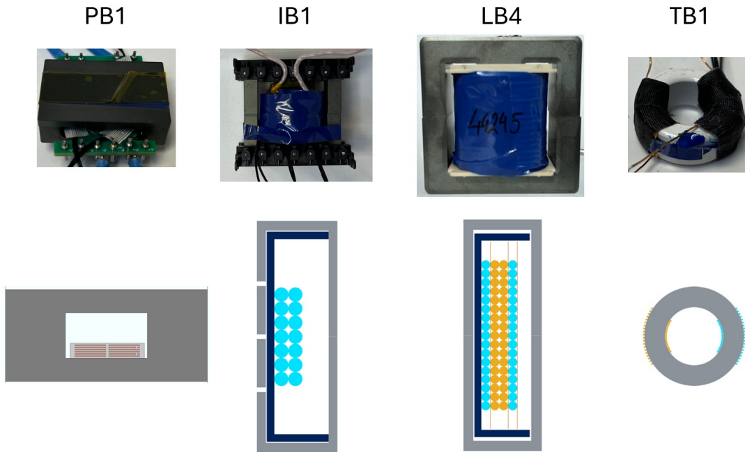
Figure 2 - Transformer prototypes
