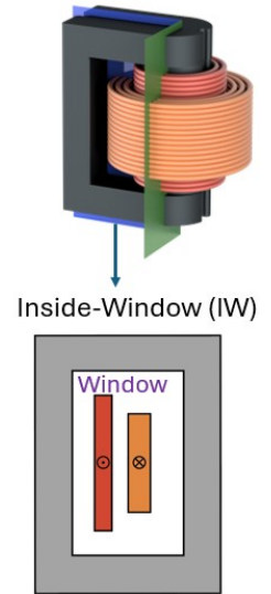
Figure 1 - Inside-Window (IW) cross section
