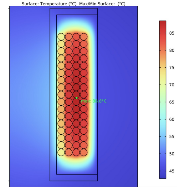
Figure 5 - Temperature distribution LB4
