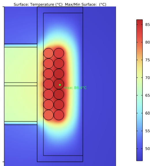
Figure 4 - Temperature distribution IB1
