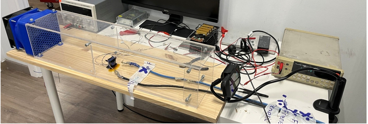
Figure 7 - Measurement Setup
