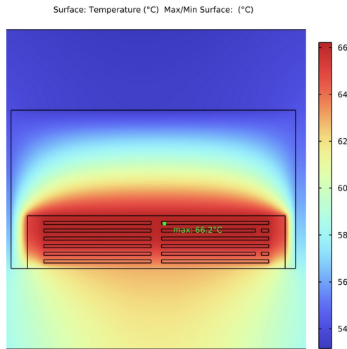
Figure 3 - Temperature distribution PB1
