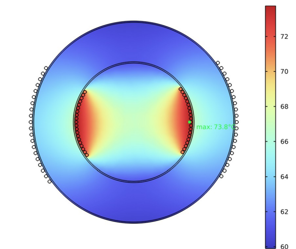
Figure 6 - Temperature distribution - TB1
