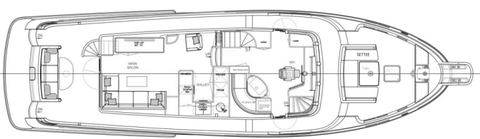
Main Deck, Galley Down
