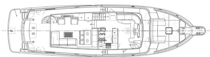
Main Deck, Galley Up
