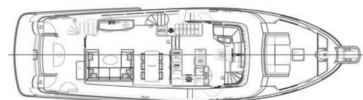
Main Deck, Wide Body Option
