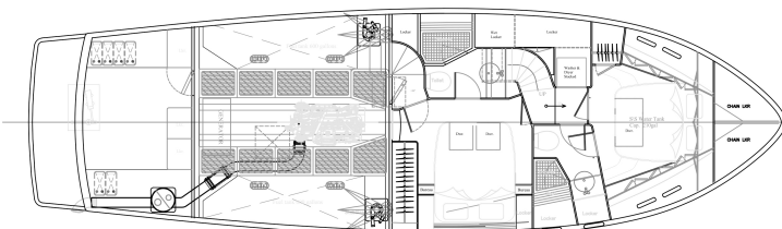
Lower Deck
