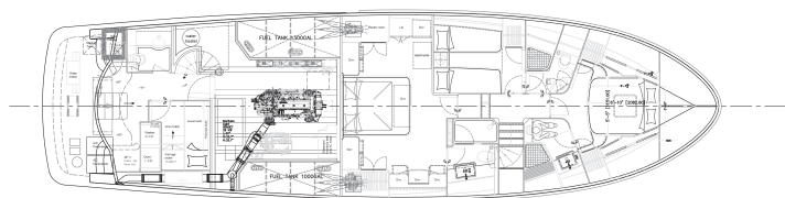
Lower Deck
