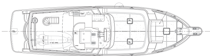
Upper Deck
