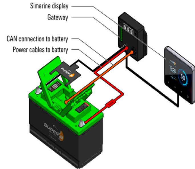
Figure 1. Typical setup
