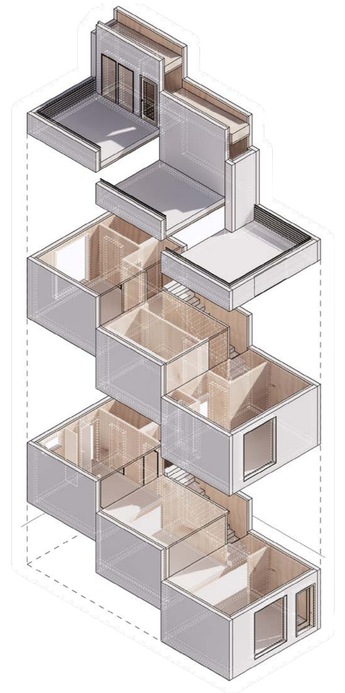
CLT Townhome Building Kit Design: Modular prefabricated elements provide for efficient delivery of a three story dwelling unit
