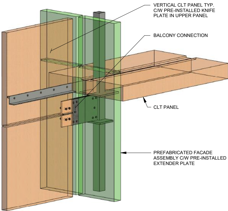
Figure 17: Structural Connection at a Column - EMTC Balconies
