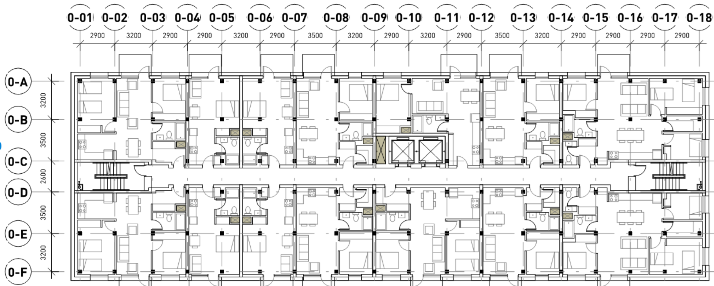
Figure 41: Slab Tower – City of Kamloops EMTC Building
