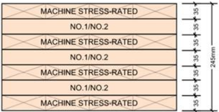
7 PLY CLT
