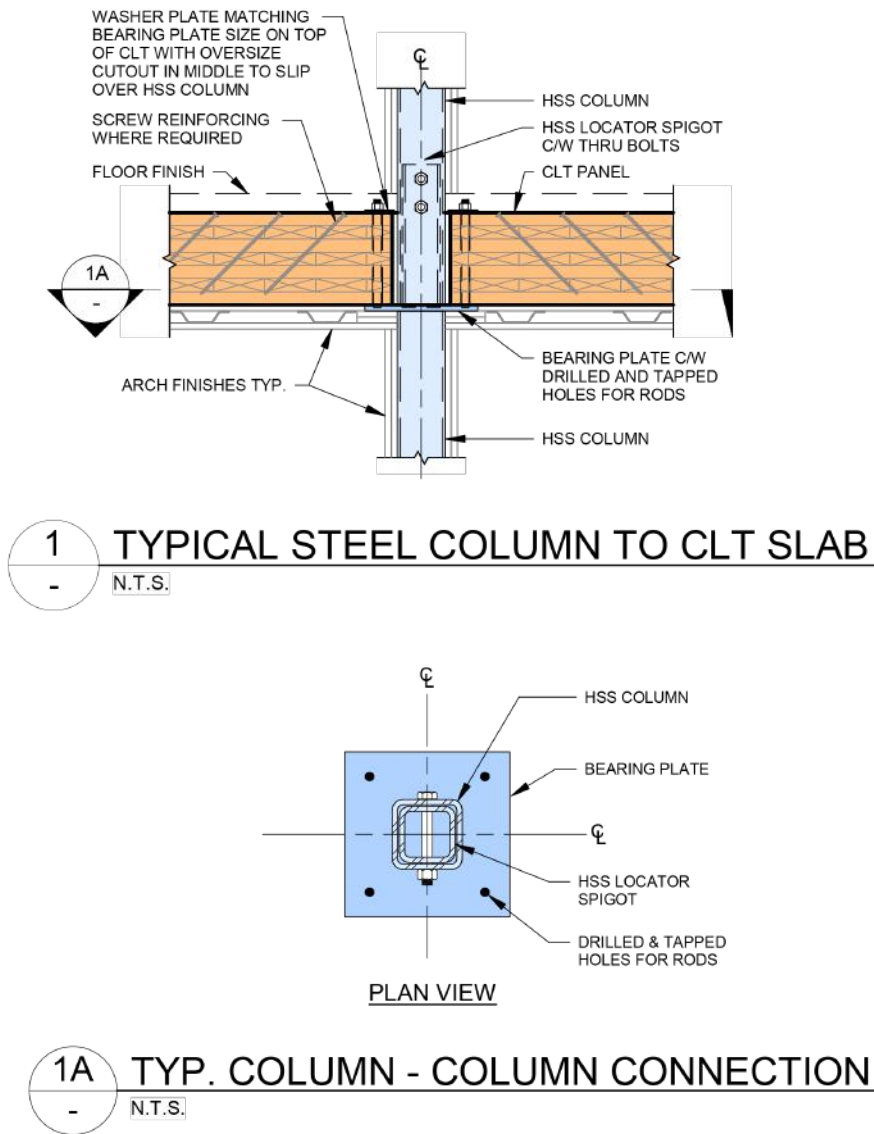
Figure 13: Typical HSS Column to Panel Connection for a CLT Point Supported System
