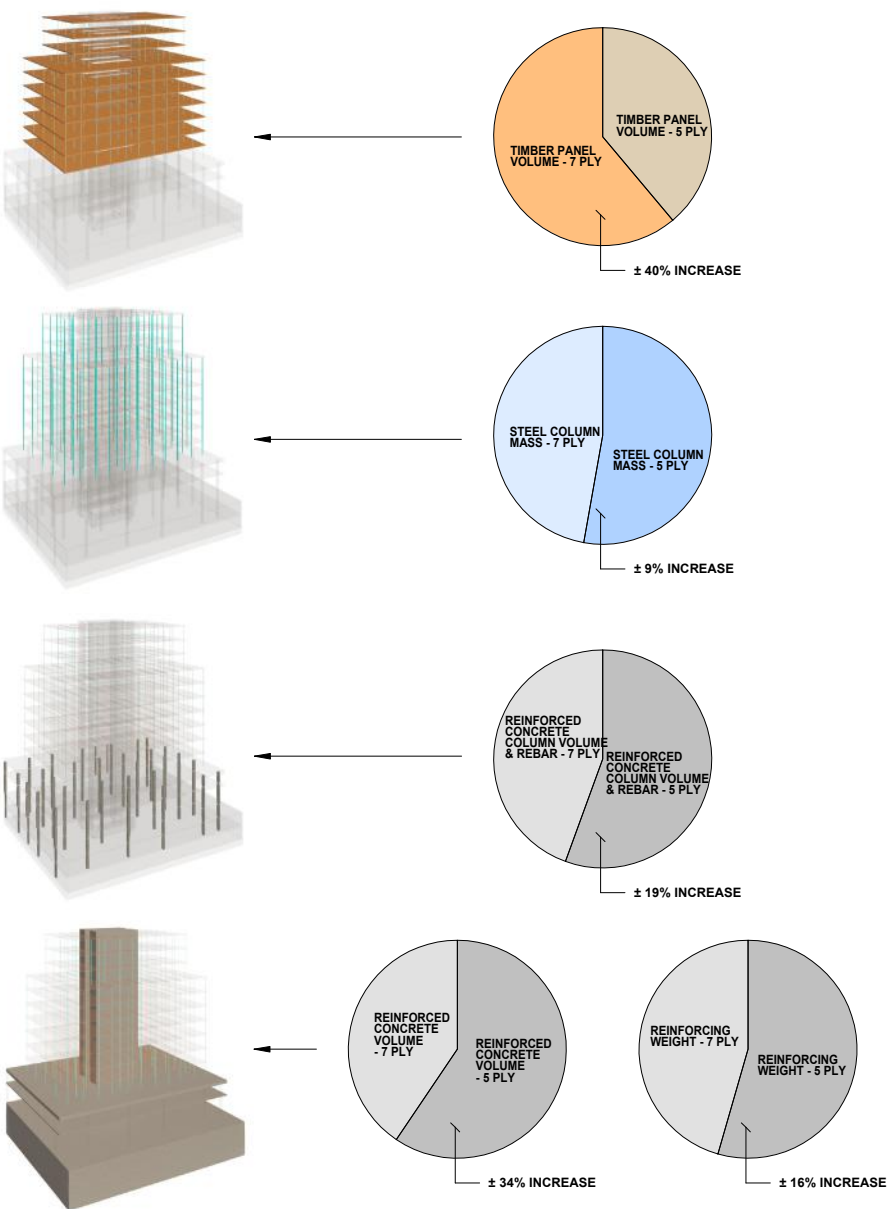
Figure 15: Comparison of a 7-ply layup vs a 5-ply layup
