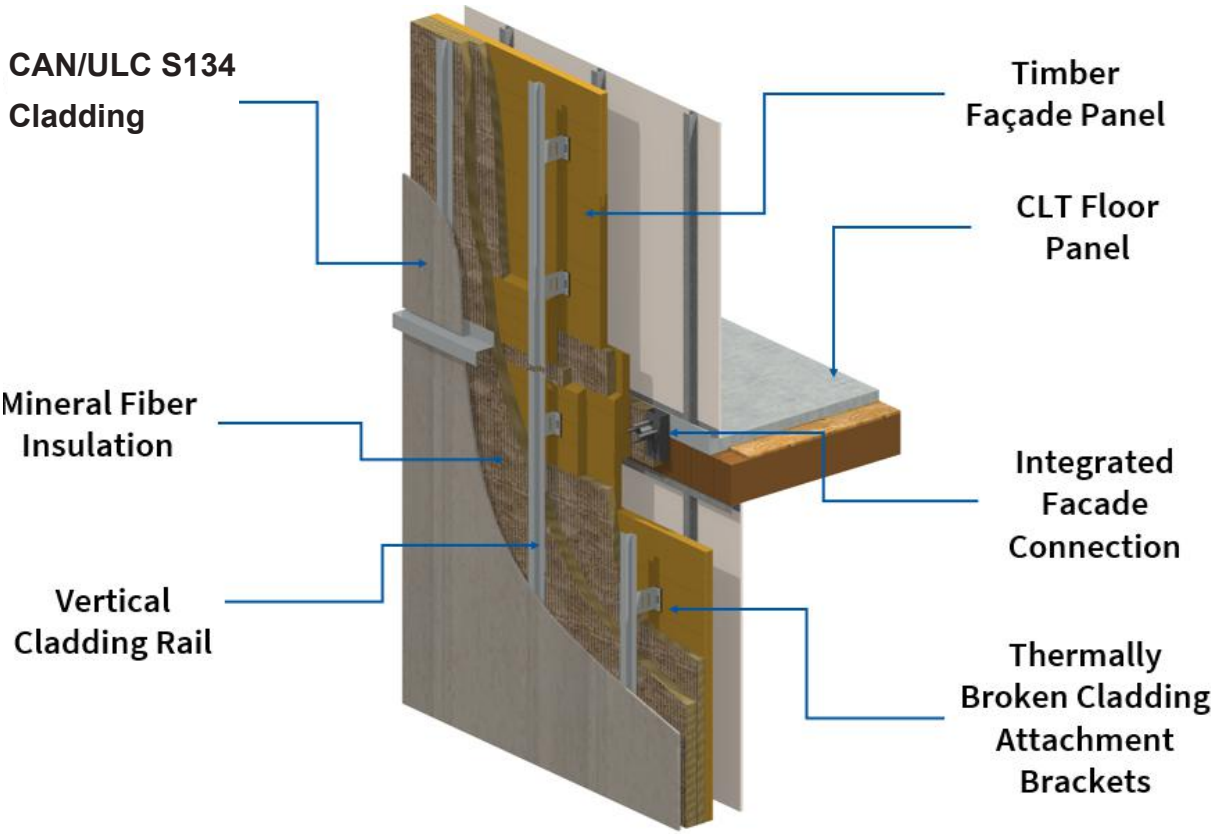
Figure 38: EMTC Facade Panel at CLT Slab Edge
