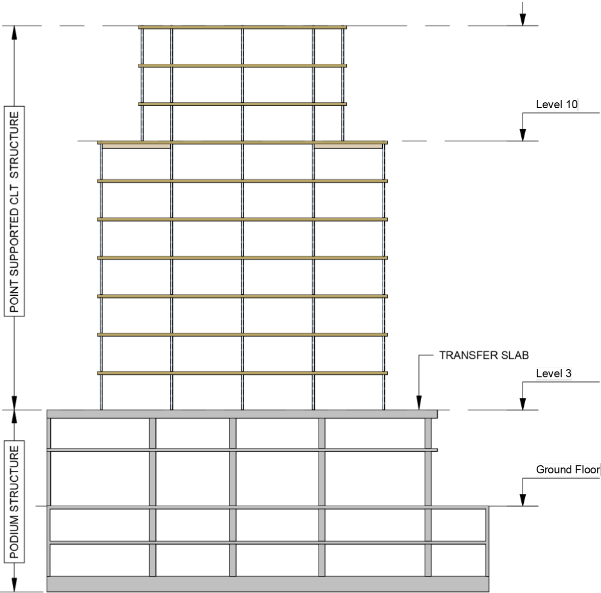
Section through the Point Tower with the podium structure:
