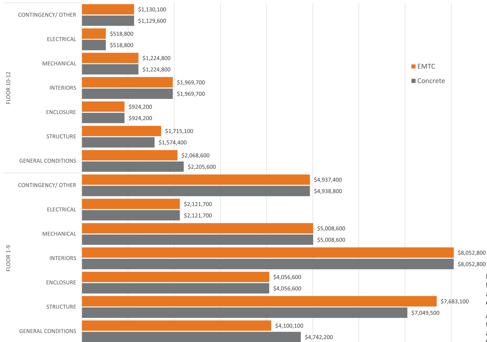
Figure 8: Slab Tower – City of Kamloops Comparison of Above Grade Floors 1-9 vs 10-12 Cost ($)
