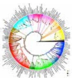
Dendrogram that displays the genetic relationships among the breeds
