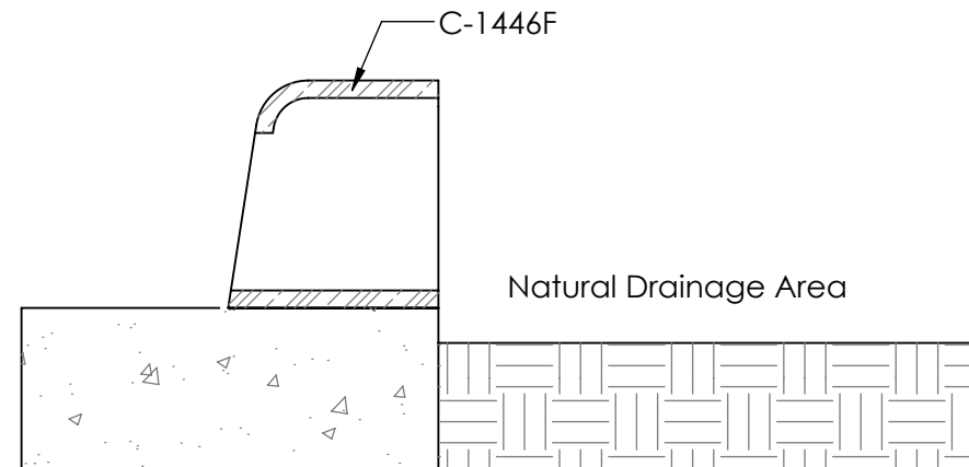
INSTALLATION DETAIL
