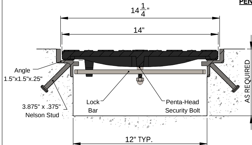
CROSS SECTION
